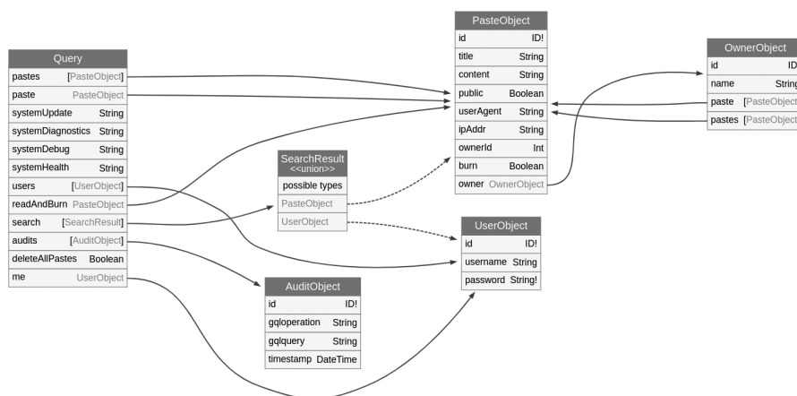
Figure 4-7: The schema view in Voyager
